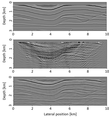
Figure 4: Loop-unrolled LSRTM on a test 2D slice of the 2D overthrust model. (a) True image, (b) RTM of simultaneous shot and (c) loop-unrolling of.
